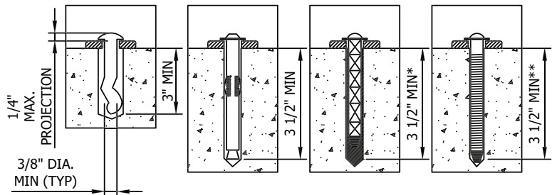
ANCHOR DETAILS
