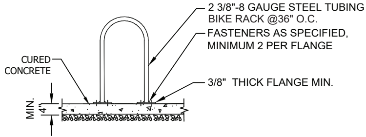
FLANGE MOUNT FLUSH (TYPICAL INSTALLATION)
